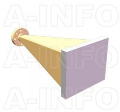
LB-15-25-ASPO Standard Gain Horn Antenna 50-75GHz 25dB Gain Rectangular Waveguide Interface
